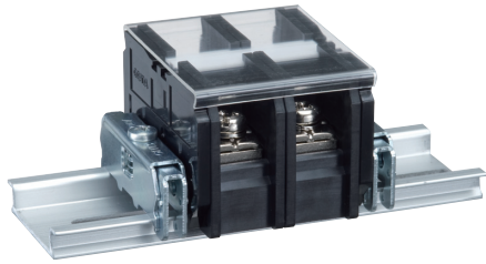
OK-11R Cover and Marking Strip (Optional)
