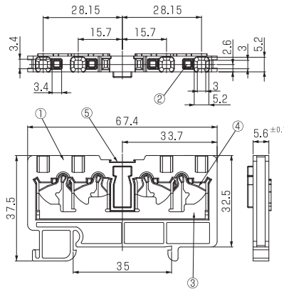
Side Plate OCN-26D-A
