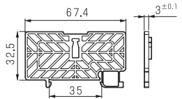
Side Plate OCN-26D-B
